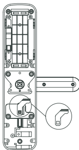
Back Side of Interior Trim for Right Open (Diagram 1)
