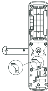
Back Side of Interior Trim for Left Open (Diagram 2)
